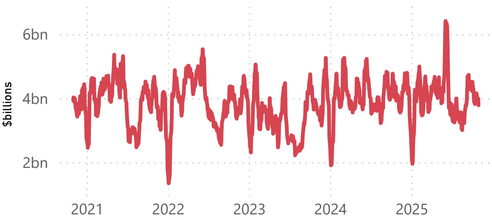
Trade Volume (10 day MA)
