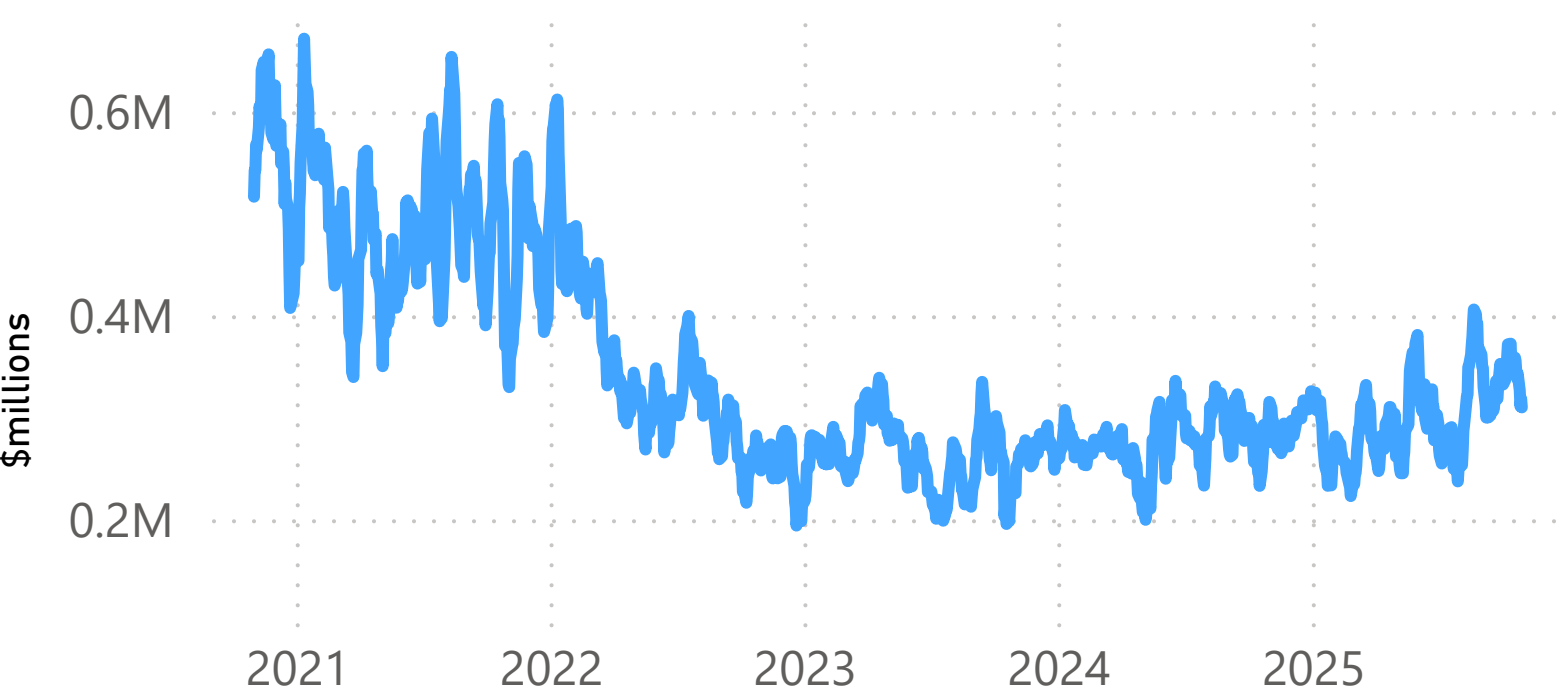
Trade Size (10 day MA)
