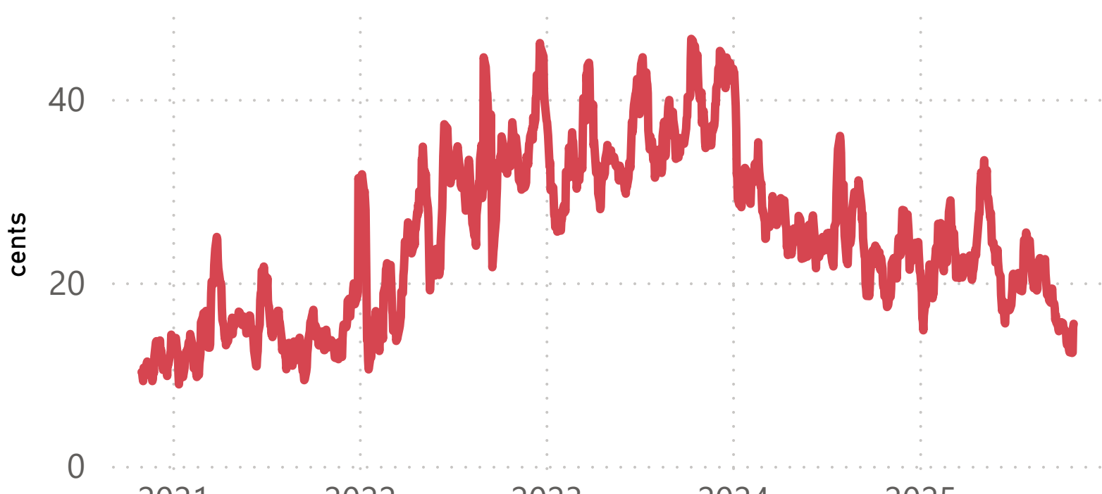
Price-Impact Proxy (10 day MA)
