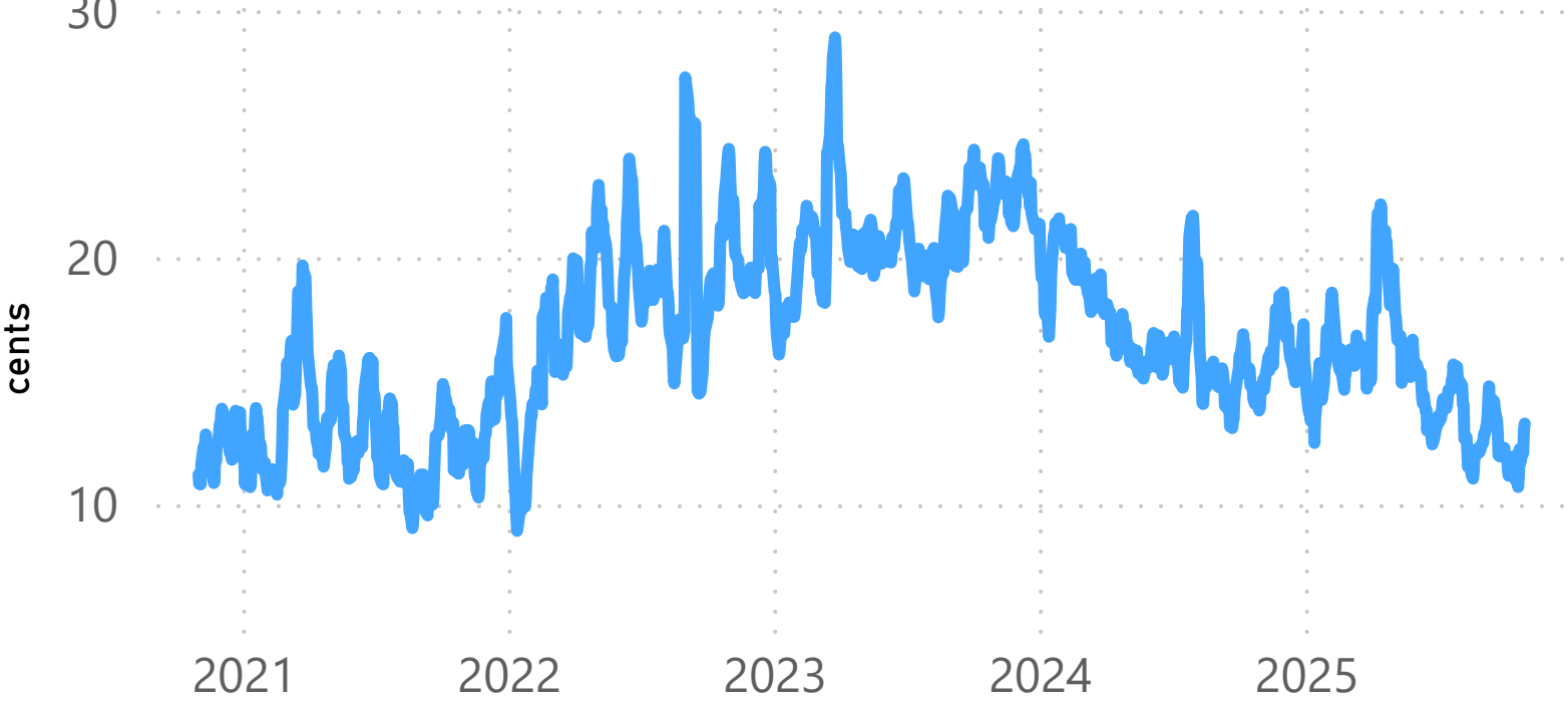
Bid-ask Spread (10 day MA)
