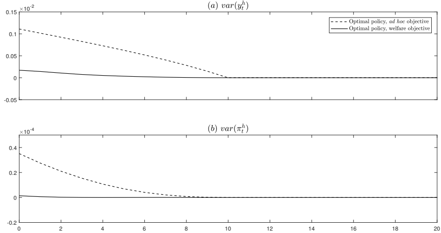
Figure 6: The paths of the dispersion measures over time, in the case of the same disturbance and same two policies as are considered in Figure 5.
