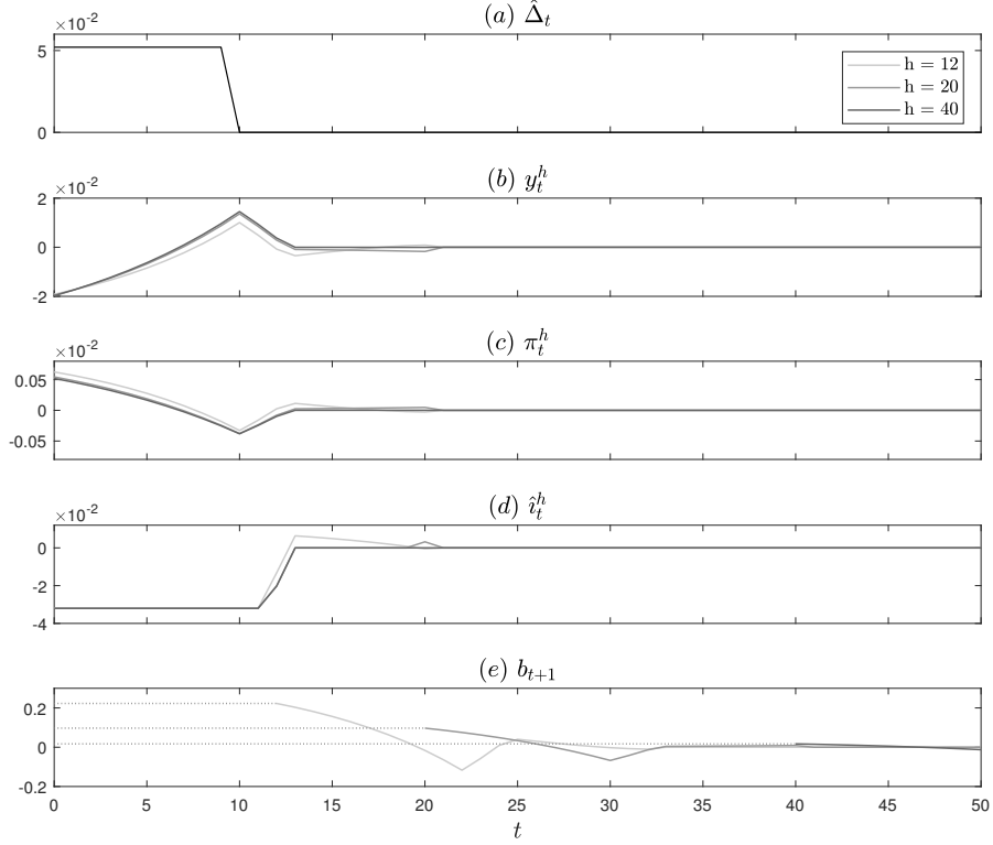
Figure C.9: Equilibrium trajectories in the case of an elevated financial wedge for 10 quarters, for households and firms with relatively long common planning horizons, under the paths of both \{b_{t+1}\} and \{\hat{i}_t\} being chosen optimally. The planning horizon h is in quarters, and t measures quarters since the onset of the elevated financial wedge.
