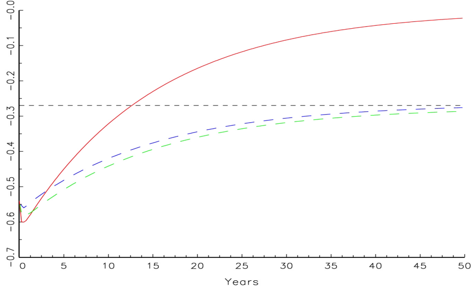
Figure 6: Future Adjustment Paths: \hat{\mathbb{E}}_T nxa_{T+k} – solid red, \hat{\mathbb{E}}_T nxa_{T+k}^T – dashed blue, \hat{\mathbb{E}}_T nxa_{T+k}^V – dashed green
