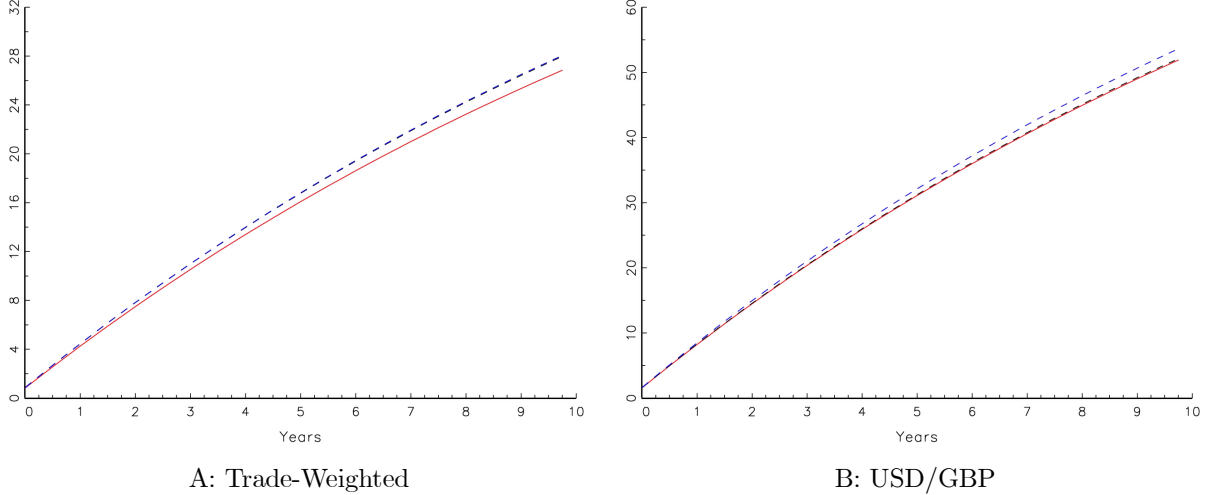
Figure 7: Expected Real Depreciation Paths using \hat{\mathbb{E}}_T nxa_{T+k} —red, \hat{\mathbb{E}}_T nxa_{T+k}^T —dashed blue, \hat{\mathbb{E}}_T nxa_{T+k}^V —dashed black
