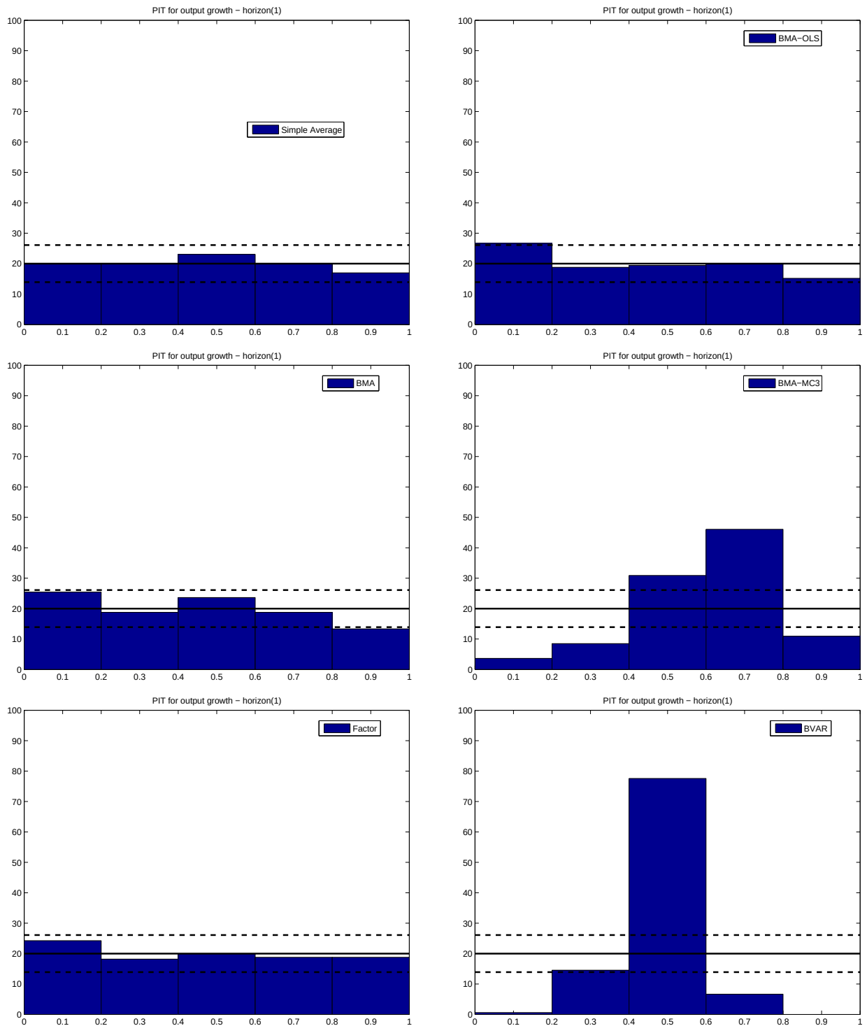
Figure 1, Panel B: PITs for Models Combining Large Data Sets of Output Growth at h = 1
